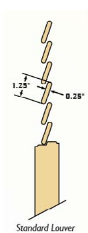
Standard Louver
